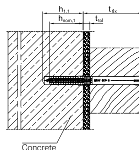
Concrete
