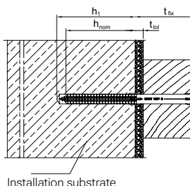
Installation substrate
